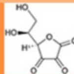
dehydroascorbic acid (oxidized form)
