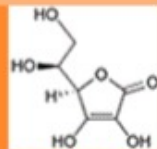
ascorbic acid (reduced form)
